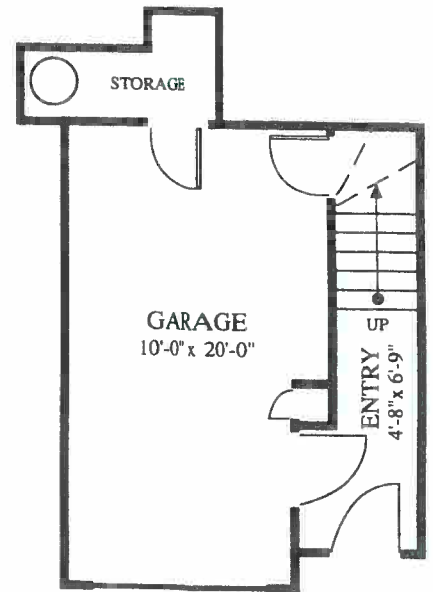
Ground Level
